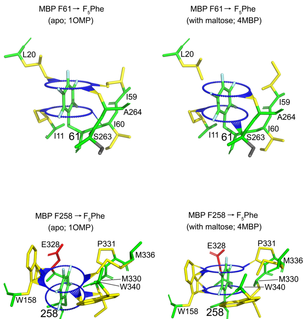
Figure S11. Modeling the ring rotation of the proteins in this work. The Phe \rightarrow F 5 Phe mutation was modeled on the crystal structures by extending the C–H bonds of the phenyl group and renaming the hydrogen to fluorine. The C 6 F 5 group was rotated in steps of 5°. Rings of blue spheres highlight the resulting fluorine positions, which display non-physical bonds in PyMOL 35 for very short inter-atomic distances, highlighting the main energy barriers for the ring rotation. The clashing atoms are listed in Table 1 of the main text. The display shows the F 5 Phe and nearby residues in a stick representation. Color code: backbone atoms and F 5 Phe residue: green (fluorine in cyan); hydrophobic side chains (Ala, Cys, Ile, Leu, Met, Phe, Pro, Trp, Val): yellow; hydrophilic side chains (Asn, Gln, Ser, Thr, Tyr): gray; negatively charged side chains (Asp, Glu): red; positively charged side chains (Arg, His, Lys): cyan. The crystal structures used were 2NUL for PpiB, 23 8QF4 for the Arc-NL/H11 complex, 28 2QMT for GB1, 36 1FKB for FKBP-12, 37 2FOM for the DENV protease, 34 2IJO for the WNV protease, 33 and 1OMP and 4MBP for MBP. 38,39
